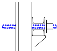
Spundwandverankerung sheet pile anchorage
