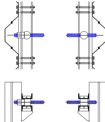
Ankergurt Verankerung waler connection
